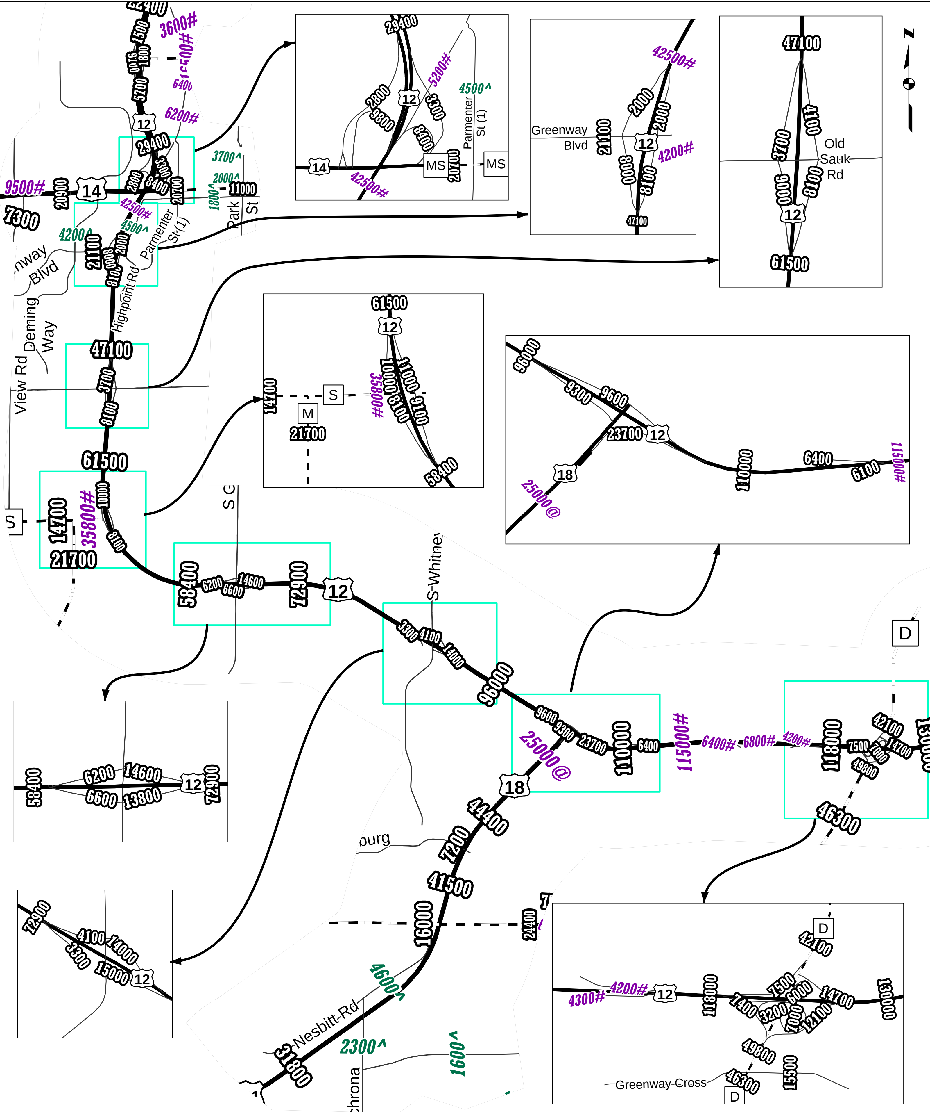
2006 BELTLINE WEST DANE County Annual Average Daily Traffic
